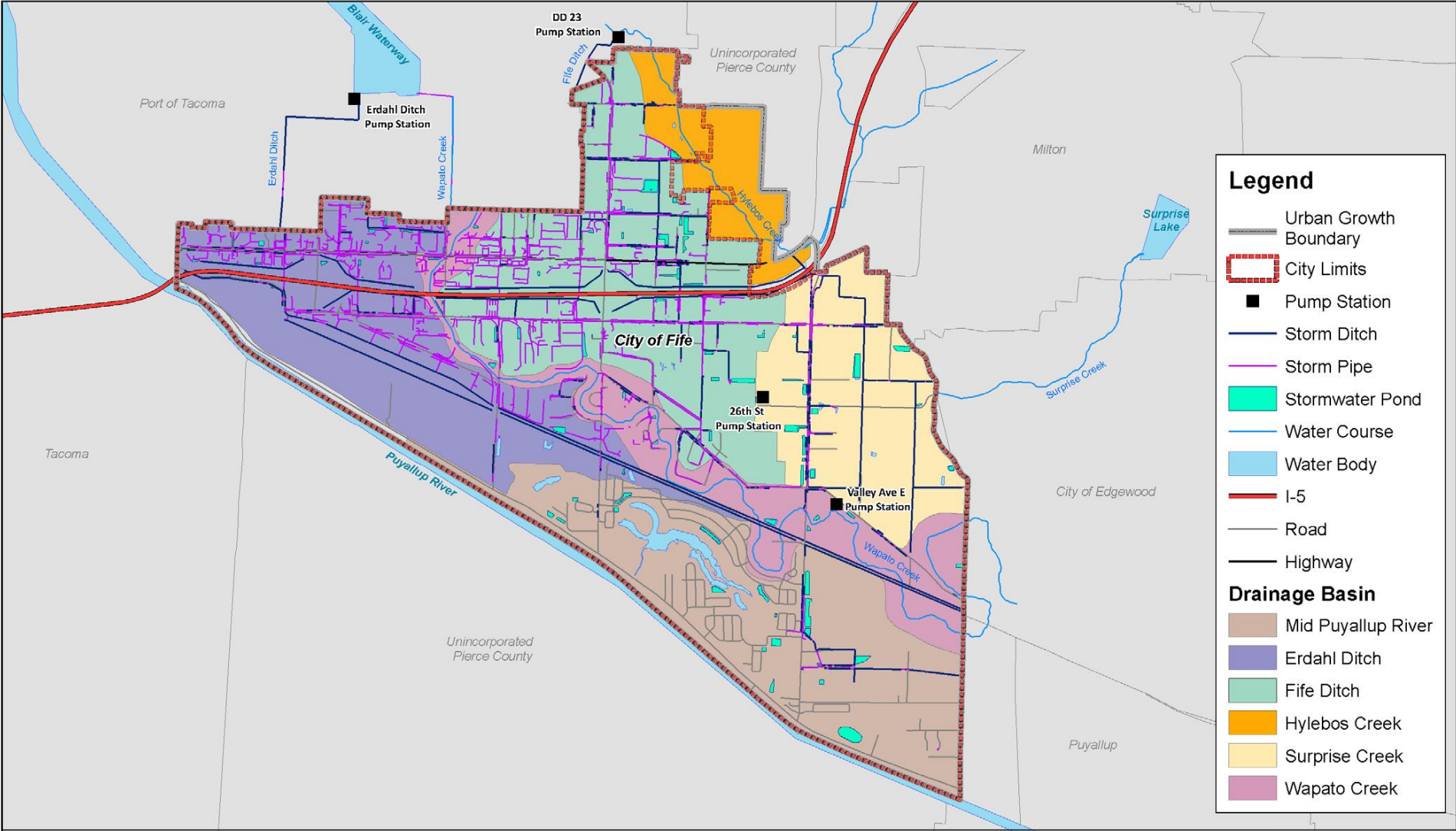
FIGURE 1 CITY OF FIFE VICINITY MAP WITH STORMWATER UTILITIES
